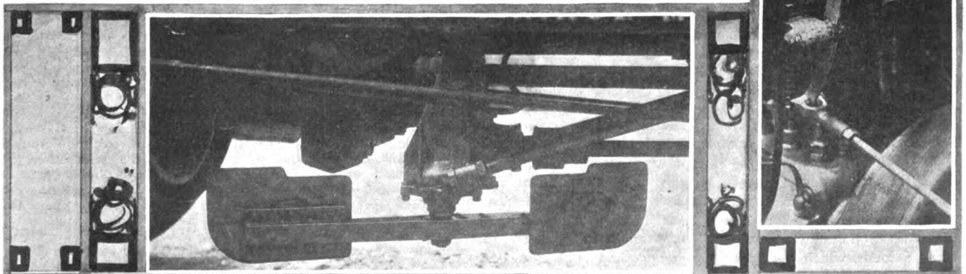
Peugeot Air Propeller Brakes Under Car Lever Control for Peugeot Brake
